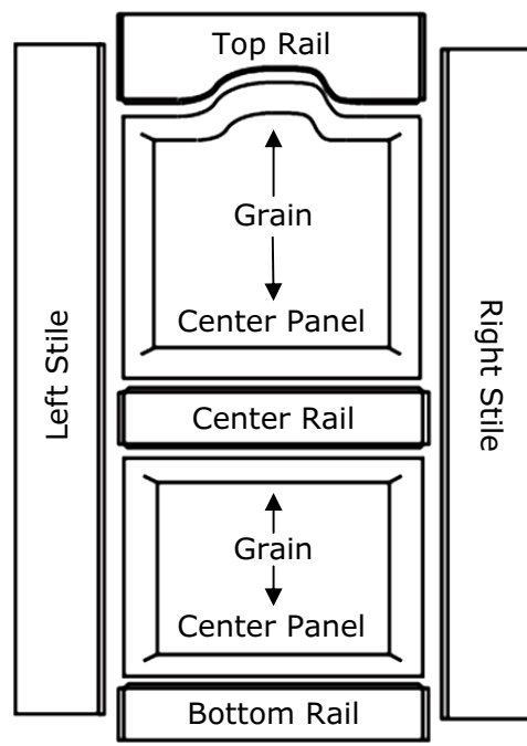
Mortise and Tenon Door
