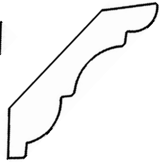
M168 H: 2 9/16" W: 2 3/8"
