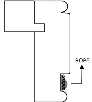
M157 H: 2 1/2" W: 1 5/8"
