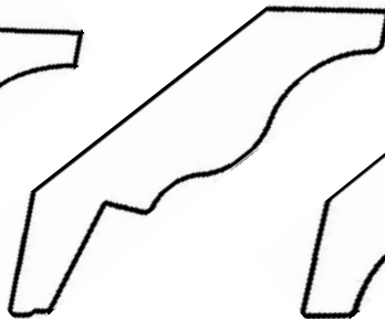
M164 H: 2 1/2" W: 2 3/8"
